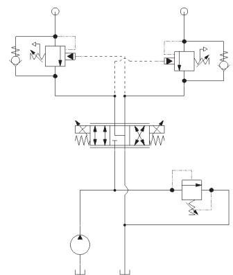
Counterbalance, Double Acting Cylinder
